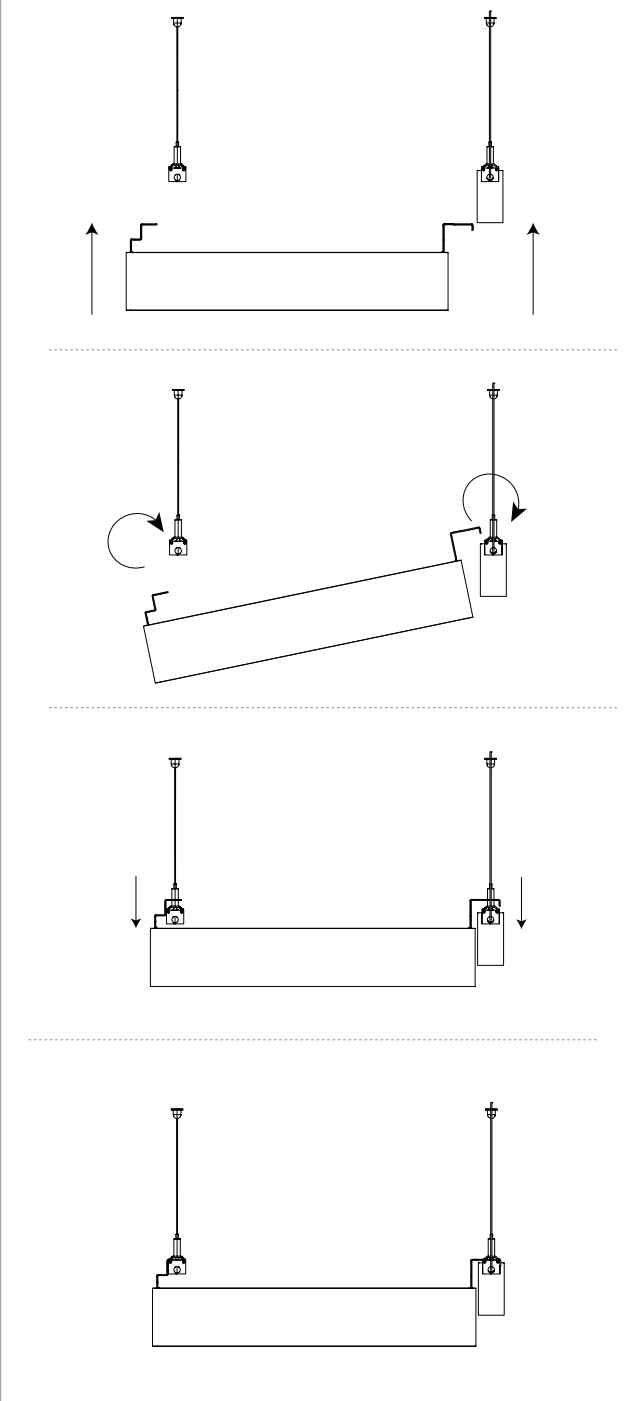
installing the frame units
