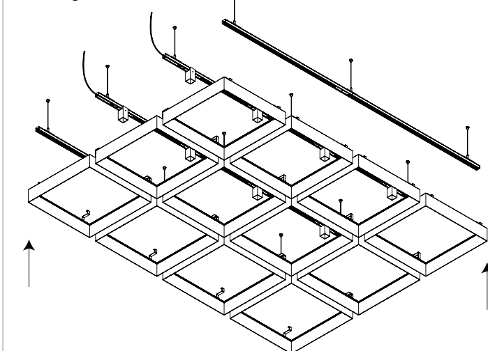
mounting the frames
