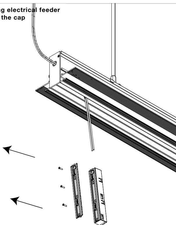
close the cap
