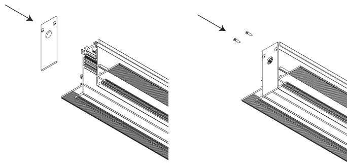
installing electrical feeder remove the cap
